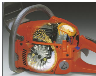
AIR INJECTION Centrifugal air cleaning system removes larger dust and debris particles before reaching the air filter. This results in reduced air filter cleanings and improved engine life.
