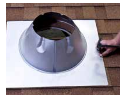
11. Slip the flashing over the roof hole so the top edge is under the shingles above. Nail the flashing to the roof across the top and down 1/2 each side. Seal flashing and nailheads with weatherizing sealant.
