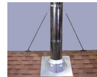
14. If the chimney is more than 5ft. above roof, support the chimney with an Extended Roof Bracket.
