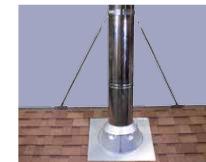
14. If the chimney is more than 5ft. above roof, support the chimney with an Extended Roof Bracket.
