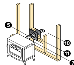
Through-the-Wall Vertical Rise
