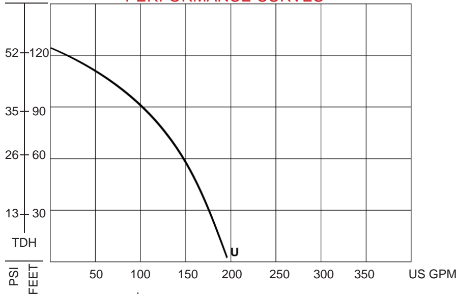
PERFORMANCE CURVES
