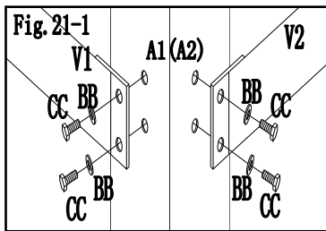
Fig.21-1: Attached Side stay (V1, V2) to Post (A1, A2) with Bolt (CC) and Flat Washer (BB).
