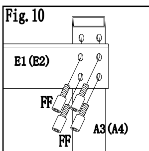
Fig.10: Install the complete back beam to back post with bolt (FF).
