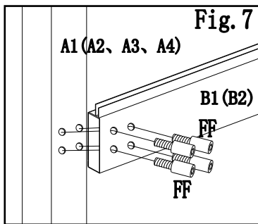
Fig.7: Use bolts (FF) to install the complete side beam 1(B1) (or side beam 2(B2)) to front post 1 (A1) and back post2 (A4)(or front post 2(A2) and back post 1(A3))
