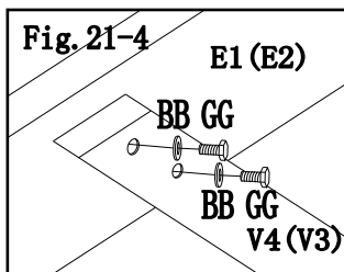
Fig.21-4: Use Bolt (GG) and Washer (BB) to lock Side Stay (V4, V3) onto Back beam (E1, E2).
