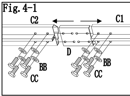
Fig.4-1: Insert the junction bar (D) into the decorative slot 1(C1) and decorative slot 2 (C2), and secure with bolt (CC) and flat washer (BB).
