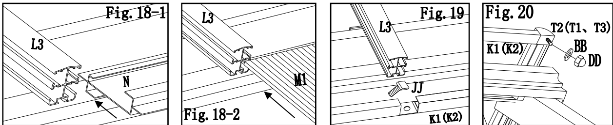
Fig.18-1: Insert the PC panel (N) into the slot of middle beam (L3), install the edge beam1 (L1) and edge beam2 (L2) the same way.
