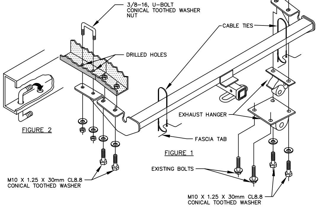
HITCH SHOWN IN PROPER POSITION
