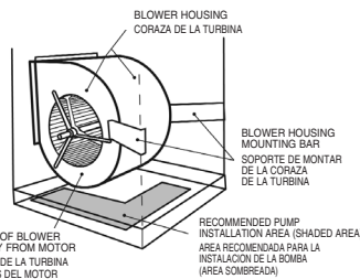
FIGURE 2. SIDEDRAFT COOLER (PARTIAL ILLUSTRATION) FIGURA 2. COOLER DE DESCARGA LATERAL (ILUSTRACION PARCIAL)
