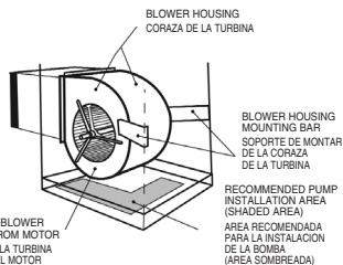
FIGURE 3. WINDOW UNIT COOLER (PARTIAL ILLUSTRATION) FIGURA 3. COOLER DE VENTANA (ILUSTRACION PARCIAL)
